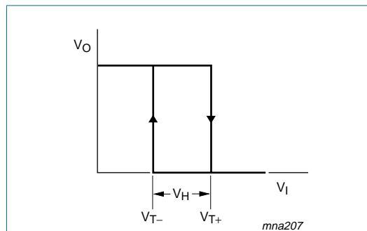
Fig 8. Transfer characteristics
