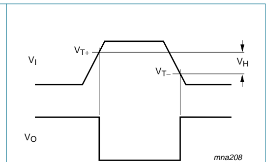
Fig 9. Definition of V_{T+} , V_{T-} and V_H
